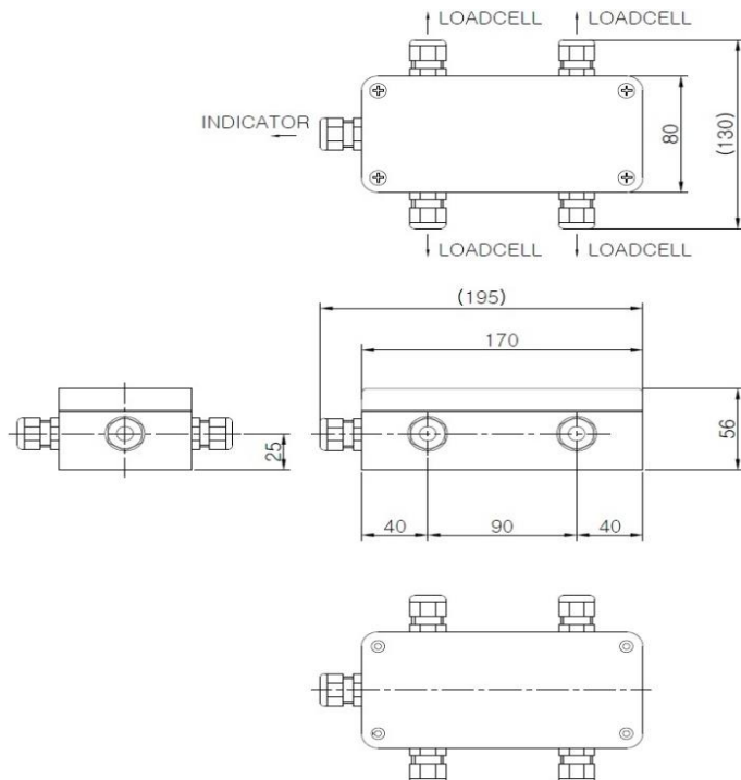
CJB-4P
