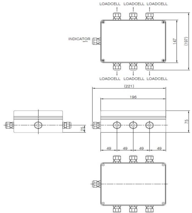
CJB-6P
